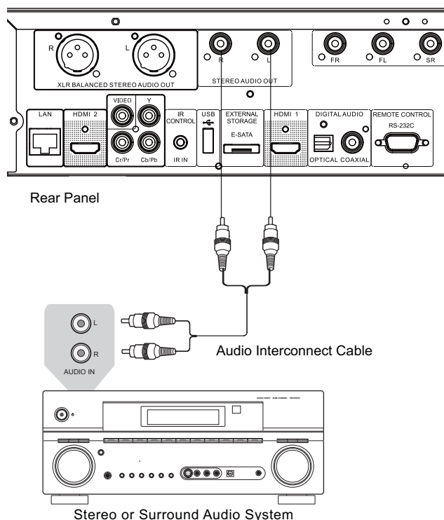
Method 7 – Stereo Analog Audio Connection by RCA cables
